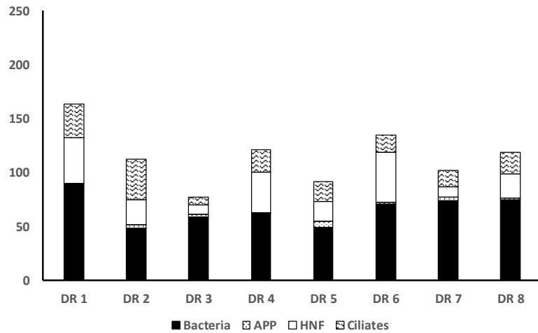
Figure 3. July 2019 planktonic food web assessment of the Detroit River Area of Concern: a) Size fractionated primary (phytoplankton) productivity including net plankton ( >20 \mu\text{m} ), nano-plankton ( 2 - 20 \mu\text{m} ) and pico-plankton ( <2 \mu\text{m} ) as well as bacterial (Bact) productivity; b) Microbial Loop and ciliate biomass (APP = autotrophic picoplankton, HNF = heterotrophic nanoflagellates, others as indicated); c) phytoplankton biomass and composition (Cyano = Cyanophyta, Chloro = Chlorophyta, Chryso = Chrysophyceae, Diatom = Diatomeae, Crypto = Cryptophyceae, Dino = Dinophyceae), and d) Zooplankton biomass and composition (clad = cladoceran, all others as indicated).
