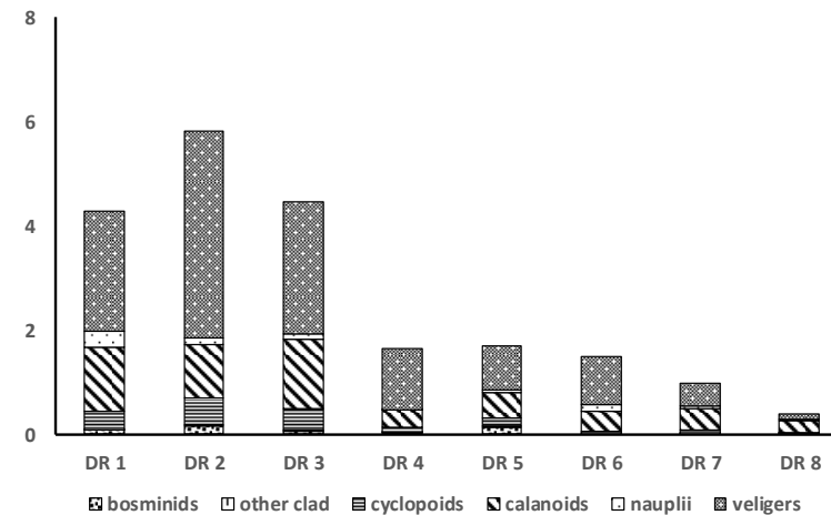
d) Zooplankton Biomass ( \text{mg m}^{-3} dry weight) and Composition
