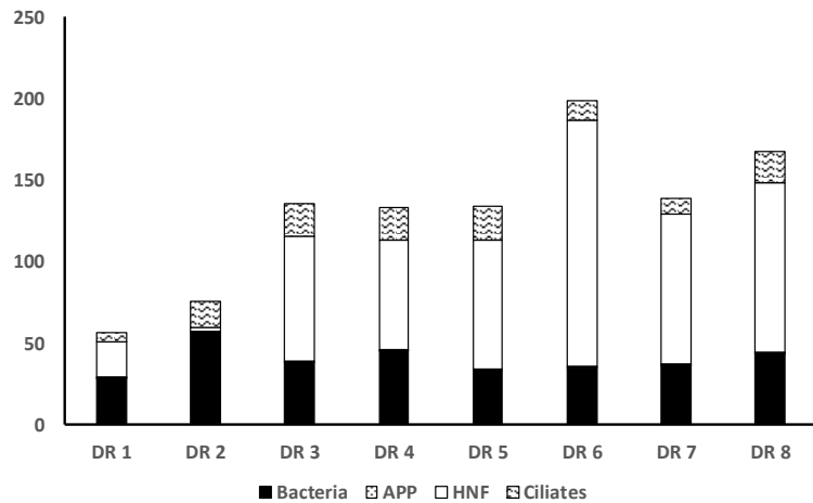
b) Microbial Loop (APP, HNF, Bacteria) and Ciliate Biomass ( \text{mg m}^{-3} )
