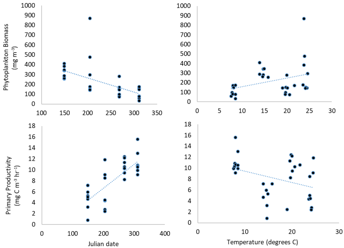
Figure 8. Relationship between a) Phytoplankton Biomass ( \text{mg m}^{-3} ) and Julian Date b) Phytoplankton Biomass ( \text{mg m}^{-3} ) and temperature ( ^{\circ}\text{C} ) c) Primary Productivity ( \text{mg C m}^{-3} \text{hr}^{-1} ) and Julian Date and d) Primary Productivity ( \text{mg C m}^{-3} \text{hr}^{-1} ) and temperature ( ^{\circ}\text{C} ).
